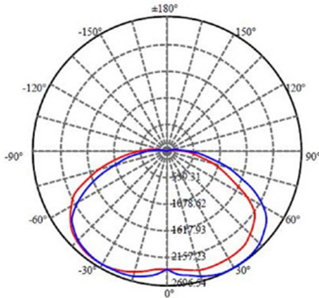
Luminous Intensity Distribution Diagram Light Distribution Curve [Unit:cd]
