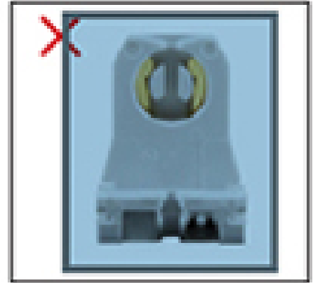
Shunted(Instant Start Socket)
