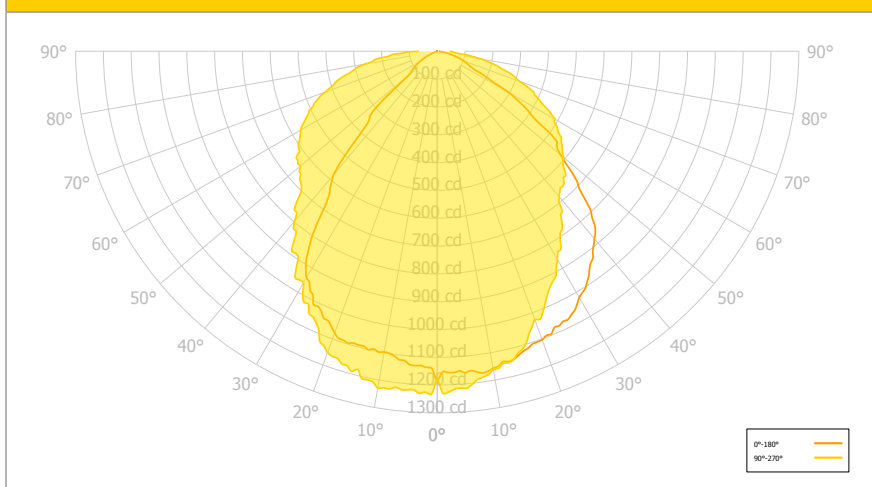
Candela Polar Plot
