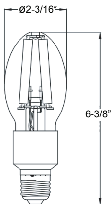
HiLED ED28 Bulb with EX39/E39 Base HiLED45S-8XX-EX39
