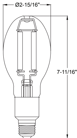
HiLED ED23.5 Bulb with E26 Base HiLED20-8XX-E26
