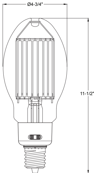
HiLED ED37 Bulb with EX39/E39 Base HiLED65S-8XX-EX39 & HiLED85S-8XX-EX39
