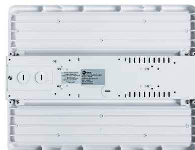
POWER & CCT SELECTABLE SWITCH
