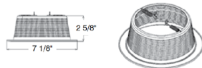
RT602BL/WH/AT Socket Supporting Black Step Baffle with White Ring, Airtight, Torsion Springs, for Floating Medium Base Socket Uses BR/PAR30 Lamps Order Code: T79610
