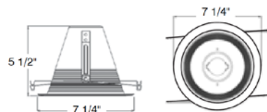
RT602BL/WH/AT Socket Supporting Black Step Baffle with White Ring, Airtight, Torsion Springs, for Floating Medium Base Socket Uses BR/PAR30 Lamps Order Code: T79610
