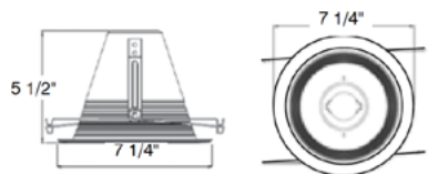
RT602GW/AT Socket Supporting Gloss White Step Baffle with White Ring, Airtight, Torsion Springs, for Floating Medium Base Socket Uses BR/PAR30 Lamps Order Code: T77565
