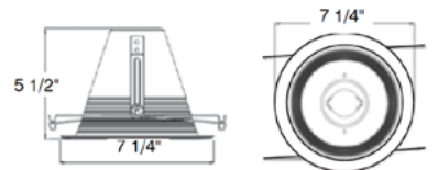
RT602GW/AT Socket Supporting Gloss White Step Baffle with White Ring, Airtight, Torsion Springs, for Floating Medium Base Socket Uses BR/PAR30 Lamps Order Code: T77565
