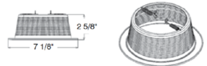
RT602BL/WH/AT Socket Supporting Black Step Baffle with White Ring, Airtight, Torsion Springs, for Floating Medium Base Socket Uses BR/PAR30 Lamps Order Code: T79610
