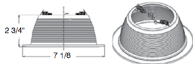
RT601WH White Step Baffle with White Ring Uses BR/PAR30 Lamps Order Code: T79135
