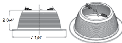
RT601BL/WH Black Step Baffle with White Ring Uses BR/PAR30 Lamps Order Code: T77102
