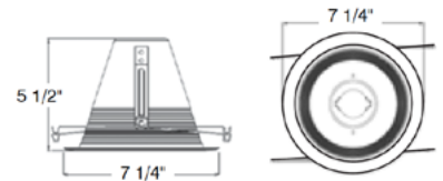
RT602BL/WH/AT Socket Supporting Black Step Baffle with White Ring, Airtight, Torsion Springs, for Floating Medium Base Socket Uses BR/PAR30 Lamps Order Code: T79610
