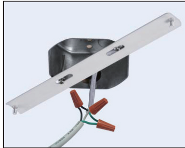
Step 2 1. Connect live supply wire (A) (typically black or the smooth, unmarked side of the two-conductor wires) to live fixture lead (B) with appropriately sized twist-on connector. 2. Connect neutral supply wire (C) (typically white or the ribbed, marked side of the two-conductor wires) to neutral fixture lead (D). 3. For positive grounding in a 3-wire electrical system, fasten the fixture ground (E) (typically cooper or green plastic coated) to the fixture mounting strap (1) with the ground screw (2).
