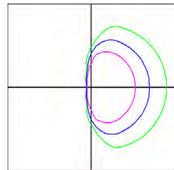
30' Mounting Height & 45° Tilt
